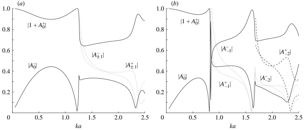
FIGURE 2. Absolute values of the amplitudes of the scattered waves plotted against ka when a/R = 0.2 for the two cases (a) \chi = \pi/2 and (b) \chi = \pi/3 .
