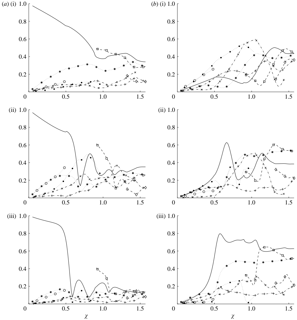
FIGURE 3. Absolute values of the amplitudes of (a) the reflected and (b) transmitted scattered waves plotted against \chi . (i) docks; (ii) stiff plates ( \gamma = 0.02 ); (iii) elastic plates ( \beta = \gamma = 0.02 ). Symbols for |A_m^\pm| : \circ , m = -5 ; \bullet , -4 ; \times , -3 ; + , -2 ; * , -1 ; \square , 1 ; \diamond , 2 .
