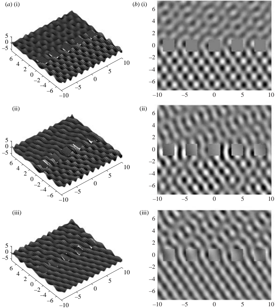
FIGURE 4. Solutions of the scattering by an array of (i) docks, (ii) stiff plates ( \gamma = 0.02 ) and (iii) elastic plates ( \beta = \gamma = 0.02 ) for an incident angle of \chi = \pi/5 . (a) side view; (b) plan view.
